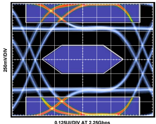
Figure 11. Tx Eye Diagram at TP2, PE = 6 dB
