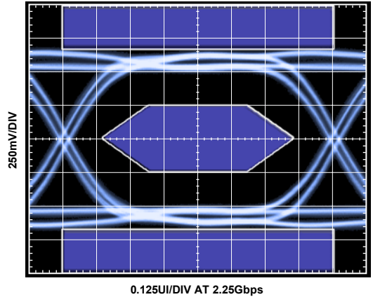
Figure 10. Tx Eye Diagram at TP2, PE = 2 dB
